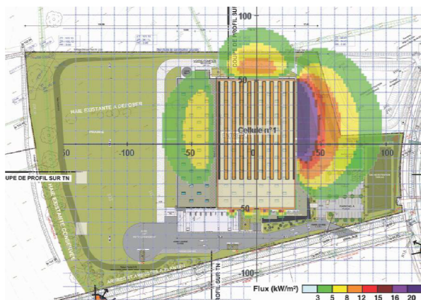
Figure 6 : FLUMILOG Cellule 1 2662
